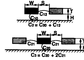
Fig. 7. Notation for coupling capacitances.
