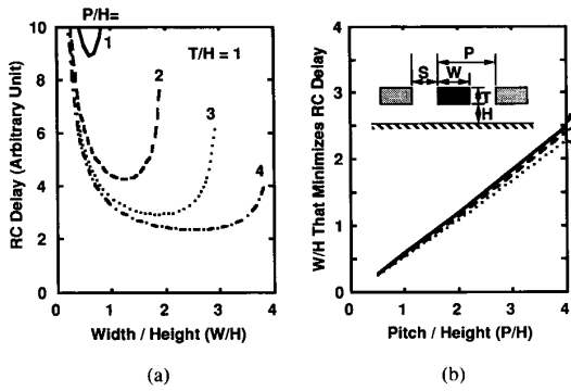
Fig. 8. (a) RC delay versus linewidth, and (b) optimum linewidth that minimizes RC delay versus pitch of the lines.
