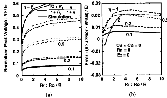
Fig. 13. (a) Peak crosstalk voltage ( R_T \neq 0 case) and (b) error of a simple expression.
