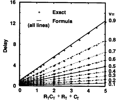
Fig. 6. Comparison of exact delay with a simple formula.
