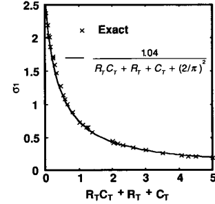
Fig. 4. Comparison between the exact value of \sigma_1 and a simple formula.
