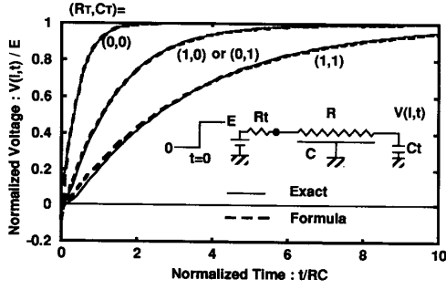
Fig. 5. Voltage waveforms of a distributed RC line.
