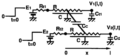
Fig. 10. Notation for capacitively coupled RC lines.
