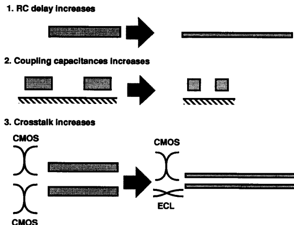
Fig. 1. Three major interconnection problems in scaled-down VLSI's.
